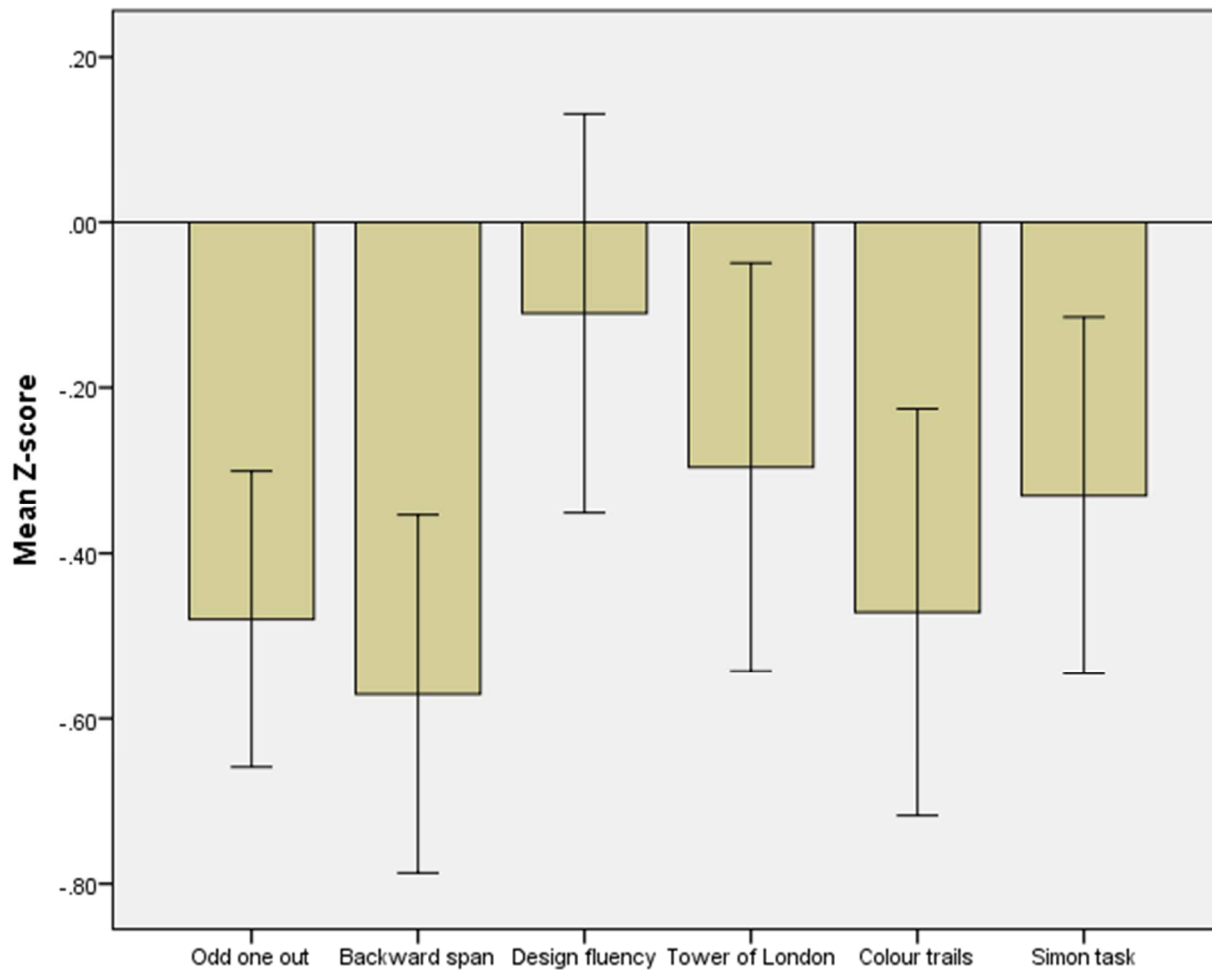
Figure 1: Mean Z-score (95% CI) on each task for children in the deaf group (based on the hearing group mean Z=0 )
