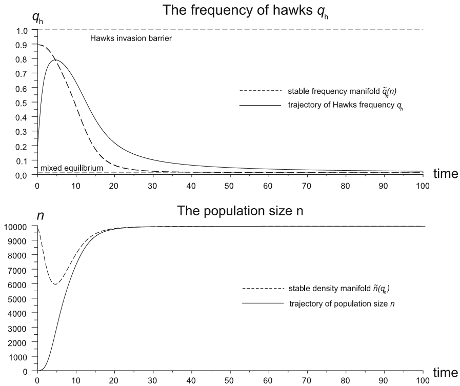
Fig. 1 The Hawk frequency increases in low population size but decreases in high population size. This is caused by newborn mortality increasing with population growth, thus making the Hawk strategy not profitable when the population size is large. Parameter values are W = 5, W_b = 0, d = 0.8, b = 0.99 [initial conditions n(0) = 20, q_h(0) = 0.2 ]. The system converges to the mixed equilibrium \check{q}_h = 0.0126 , population size \tilde{n} = 9,959 , where the Hawk invasion barrier is \hat{q}_h = 0.9974
