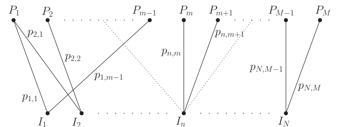
Fig. 1. Representing an independent model as a bi-partite graph where the weight between the vertex representing individual I_n and place P_m is p_{n,m} .
