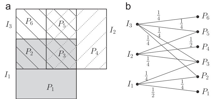
Fig. 2. Territorial interaction model. (a) The territory of individual I_1 is the square in grey, the territory of I_2 is the square encompassed by the dotted lines, the territory of I_3 is the square encompassed by full lines; (b) is the corresponding graphical representation as a general independent model.
