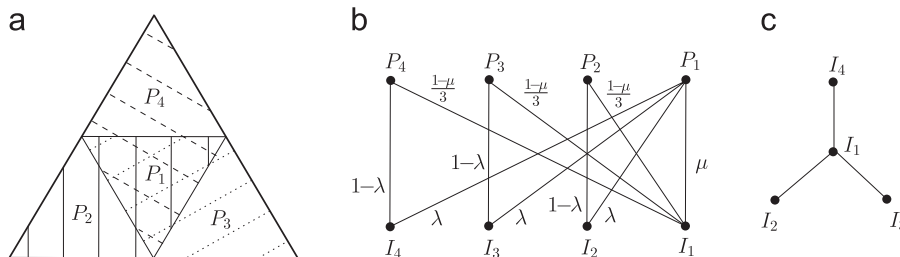
Fig. 4. The territorial raider model. (a) Individual I_n lives in place P_n but can raid neighbouring places. The territory of I_1 is the whole triangle and the home place is the central smaller triangle. The territory of I_2 is the rhombus encompassed by full lines, the territory of I_3 the rhombus encompassed by dotted lines and the territory of I_4 the rhombus encompassed by dashed lines; (b) is the corresponding graphical representation as a general independent model; and (c) is an alternative visualisation as some multi-player interactions on a graph.
