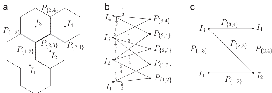
Fig. 3. The boundary interaction model. (a) Individuals are guarding their areas; (b) is the corresponding graphical representation as a general independent model; and (c) is an alternative visualisation as pairwise interactions on graphs.
