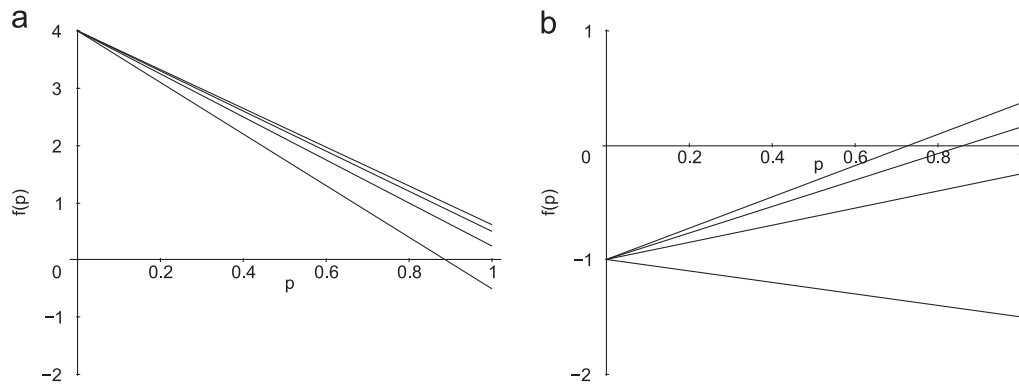
Fig. 5. Graphs of f(p) from (37) for varying d . In (a), B_H - B_I = 1, F_O = 3, L_H - L_I = 0, F_H - F_I = 0, F_I = 3 and d = 2 (bottom line), d = 4.6 (middle lines) and d = 8 (top line); here p = 0 is always an ESS, p = 1 is an ESS only if d < 3 . In (b) B_H - B_I = -2, F_O = 1, L_H - L_I = -2, F_H - F_I = -1, F_I = 5 and d = 2 (bottom line), d = 4.6 (middle lines) and d = 8 (top line); here p = 0 is never an ESS, p = 1 is an ESS only if d \leq 5 and there is a mixed ESS for d > 5 .
