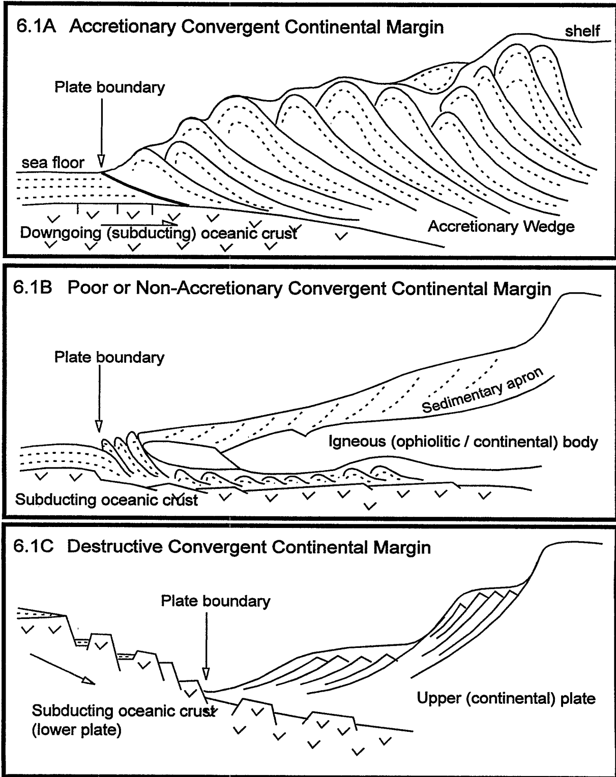
Figure 6.1: Schematic illustrations of different continental margin types
