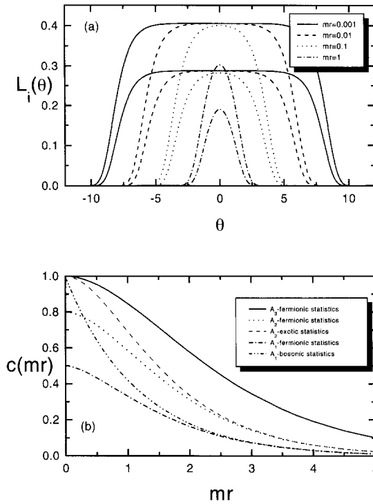
Fig. 3. Solution of the TBA equation for the A_3 -minimal affine Toda field theory (a). For the same value of mr the curve L_2(\theta) is always below L_1(\theta) . Scaling function for systems involving different types of dynamical and statistical interaction (b). The exotic statistics for A_2 means g_{ij}=\delta_{ij}-N_{ij} .
