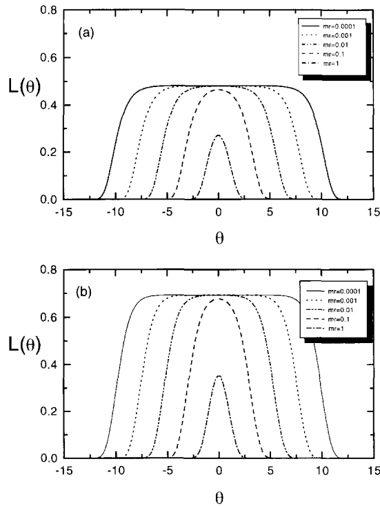
Fig. 2. Solution of the thermodynamic Bethe ansatz for the scaling Potts model with (a) fermionic statistical interaction and (b) exotic statistical interaction, i.e. g_{ij}=\delta_{ij}-N_{ij} .
