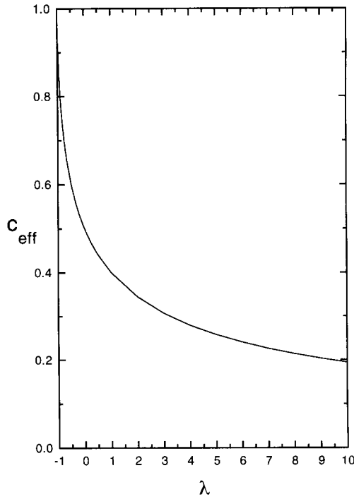
Fig. 1. The effective central charge for the ultraviolet limit of the Calogero–Sutherland model versus its coupling constant \lambda .
