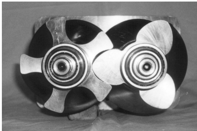
Fig 2 Expressor rotors
