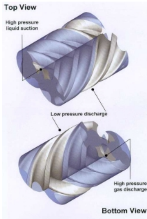
Fig. 3 Operating principle of a twin-rotor expessor
