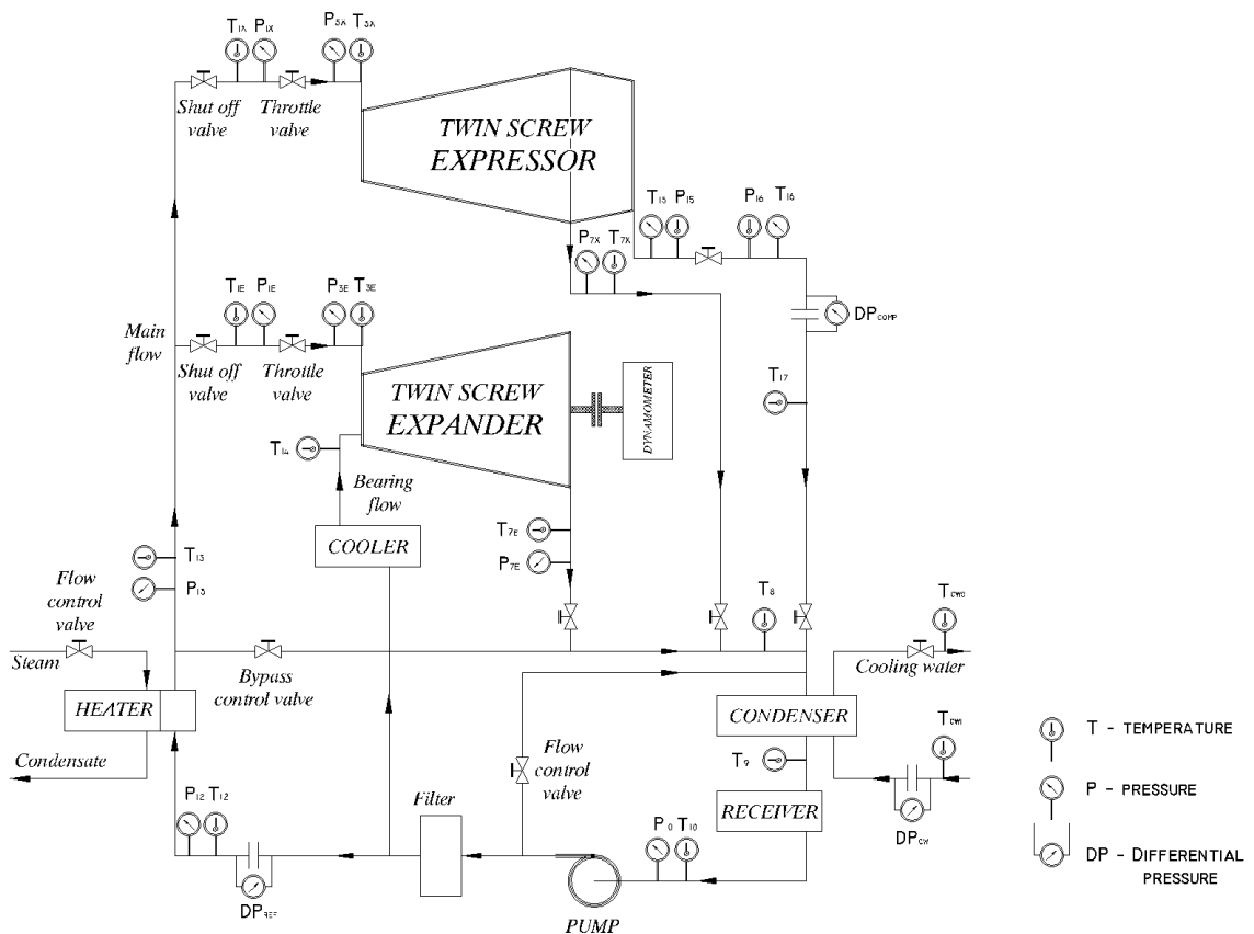
Fig 6 Layout of the expressor test rig
