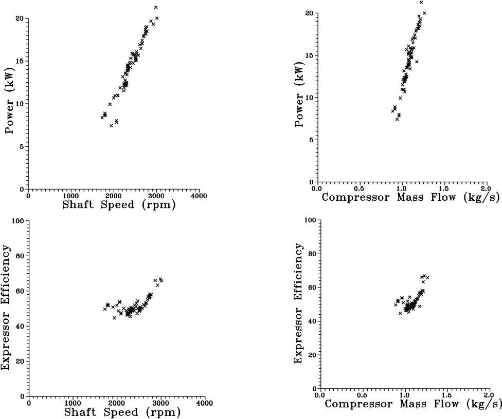
Fig 7 Expressor performance charts
