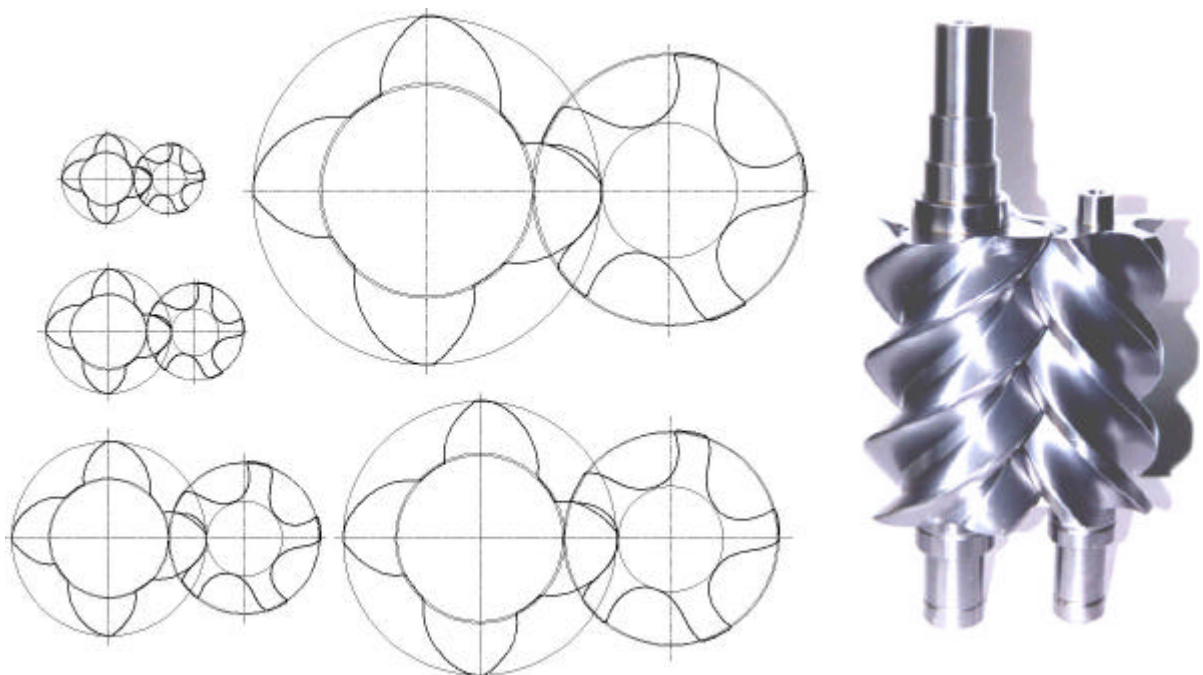
Fig 1. 4/5 'N' rotors scaled for the family of screw air compressors
