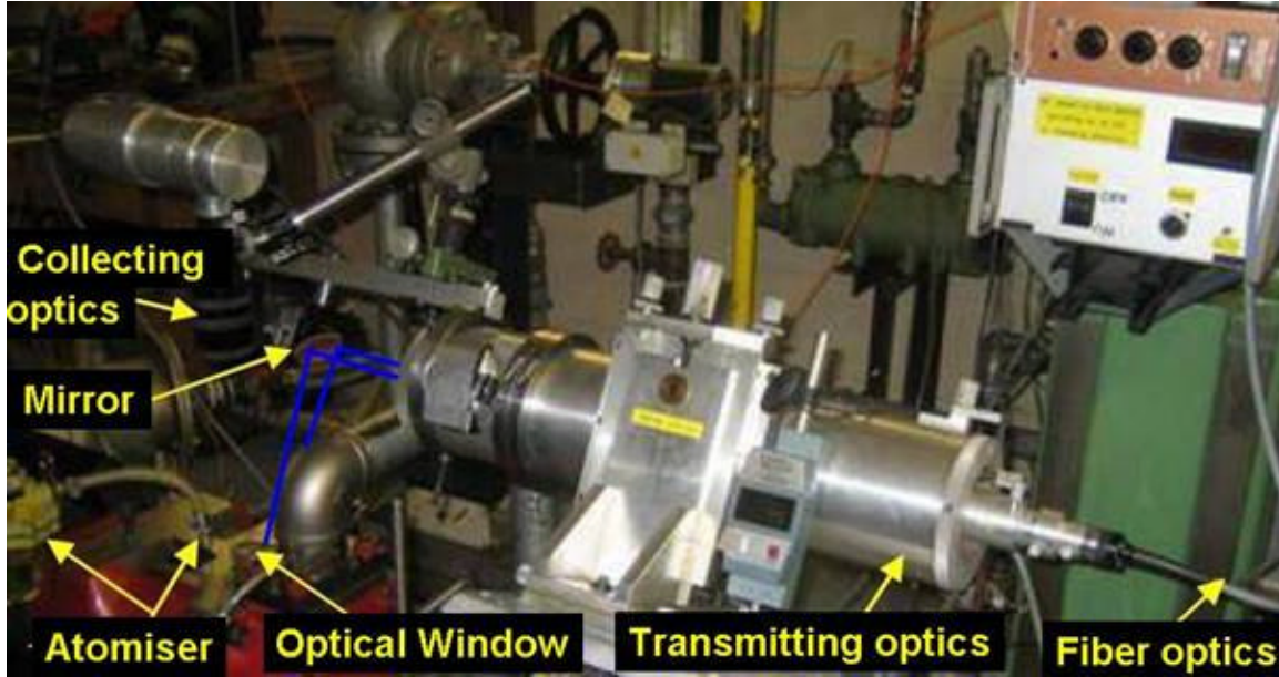
Figure 4: LDV optical set up of transmitting and collecting optics.
