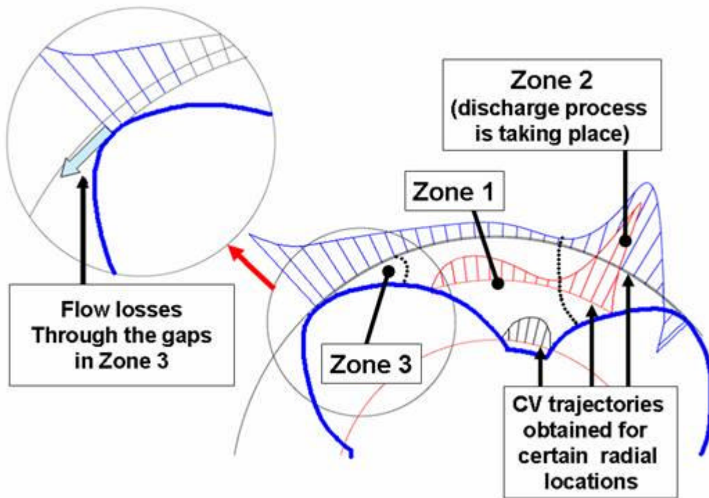
Figure 6: Schematic representation of flow structure within the interlobe region.
