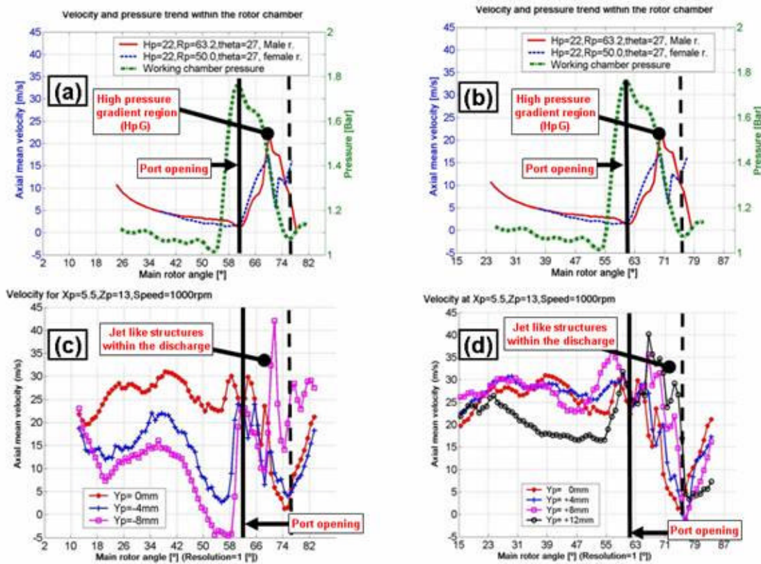
Figure 9 The effects of pressure difference on velocity fields: (a) Main rotor curves (b); Female rotor curves; (c) Outlet curves of the port region close to the main rotor, (d) Outlet curves of the port region close to the female rotor.
