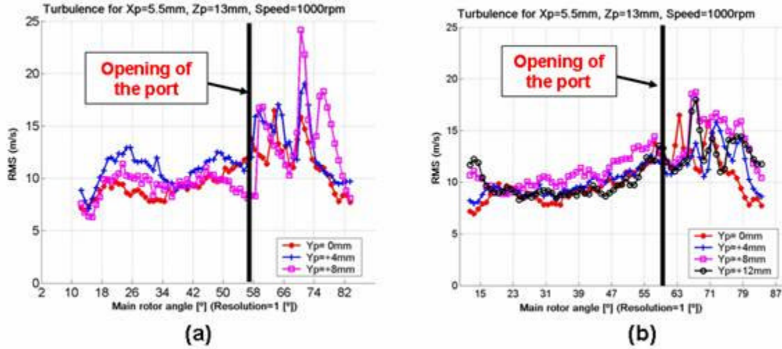
Figure 8 Axial RMS velocity variation on the outlet of the discharge port: (a) Outlet curves of the port region close to the main rotor (b) Outlet curves of the port region close to the female rotor.
