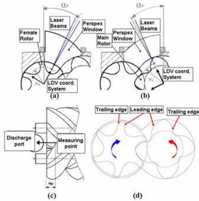
Figure 3: (a) Coordinate system and window adopted for the female rotor; (b) Coordinate system and window adopted for the male rotor; (c) Axial plane view; (d) view, of male and female rotor edges.
