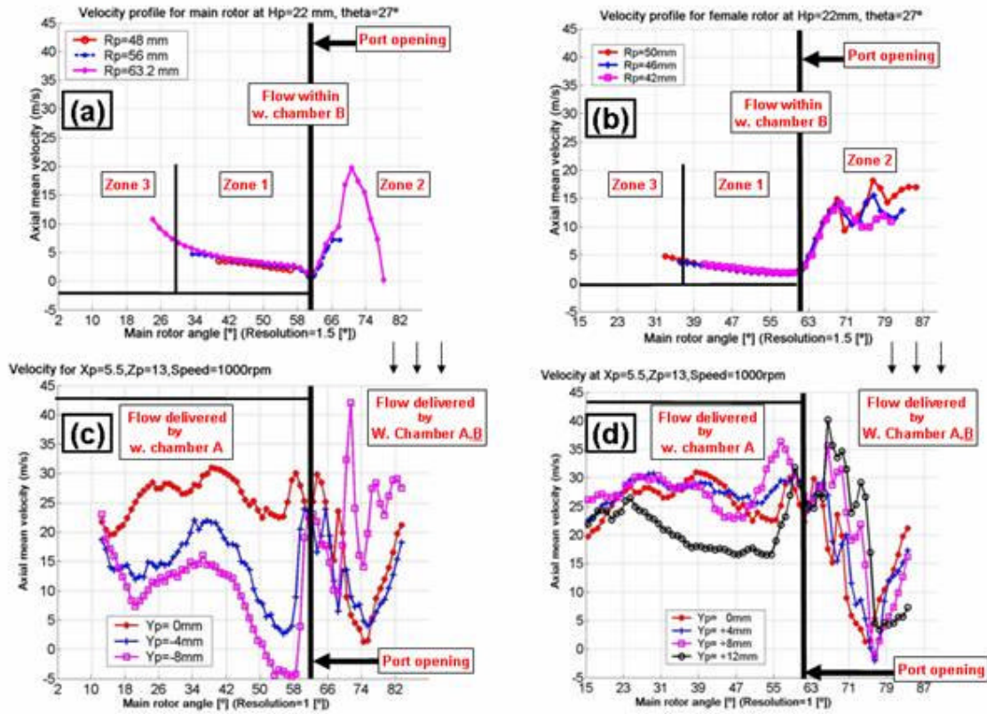
Figure 7 Comparison between discharge axial mean velocity component at the inlet (rotor side) and outlet (cavity side) of the discharge port: (a) Inlet main rotor curves (b) Inlet female rotor curves; (c) Outlet curves of the port region close to the main rotor (d) Outlet curves of the port region close to the female rotor.
