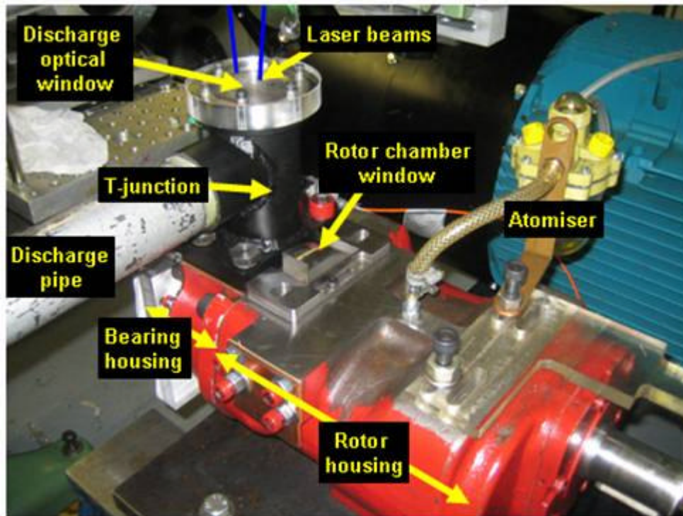
Figure 1 : Optical compressor equipped with transparent windows near the discharge;
