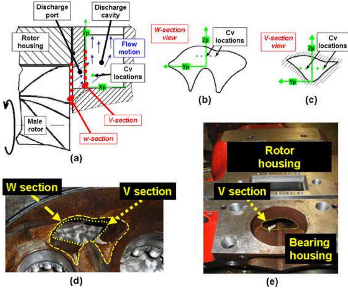
Figure 2: Geometry of the compressor at the outlet port: (a) Transverse-section of the discharge (b) W section view, (c) V section view; (d) Actual discharge port viewed from rotors side; (e) Actual discharge port viewed from cavity side
