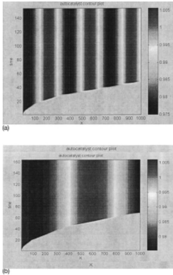
FIG. 4. (a). Gray scale contour plot of the activator concentration showing the spatial periodic pattern for the case when the flow is set away from the critical value: \delta=1.0 , \mu=0.99 , \phi=11.0 . Here \phi_{*c}^*(1.0,0.99)=9.924 . (b). Gray scale contour plot of the activator concentration showing the spatial periodic pattern for the case \delta=1.0 , \mu=0.99 , \phi=30.0 . Note the increase in the pattern wavelength with the flow as compared to that in Fig. (a).
