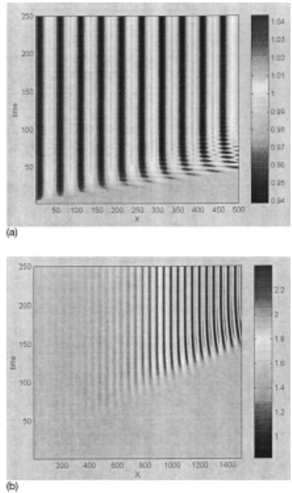
FIG. 5. (a). Gray scale contour plot for the activator species concentration b for the case \delta=4.5 , \mu=0.98 , \phi=0.39 . Here \phi_{*c}(4.5,0.98)=0.365 . (b). Gray scale contour plot for the autocatalyst concentration for the case \delta=9.26 , \mu=1.5 , \phi=0.55 . Here \phi_{*c}(9.26,1.5)=0.5035 .
