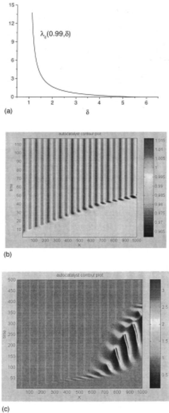
FIG. 3. (a). A plot of the analytically predicted wavelength as given by Eq. (4.2) for \mu=0.99 and for \mu^2 = 0.9801 < \delta < \delta_T = (3 + 2\sqrt{2})\mu^2 = 5.71 . (b). Gray scale contour plot of the activator concentration showing the spatial periodic pattern for the case \delta = 1.2, \mu = 0.99 . Here \phi_c^*(1.2, 0.99) = 2.98 \dots . Here \phi_{*c}(1.2, 0.99) = 0 . The wavelength of the periodic pattern is \lambda(\text{numeric}) = 20.9 and we have predicted \lambda(\text{analytic}) = 20.822 . (c). Gray scale contour plot of the activator concentration showing the spatial periodic pattern for the case \delta = 2.0, \mu = 0.99 . Here \phi_c^*(2.0, 0.99) = 1.291 \dots . Here \phi_{*c}(2.0, 0.99) = 0 . The wavelength of the periodic pattern \lambda(\text{numeric}) = 12.45 and we have predicted \lambda(\text{analytic}) = 12.442 . Note the initial dynamic structure (transient) in the concentration that is eventually washed out from the domain by the flow. A stationary periodic pattern finally invades the entire domain.
