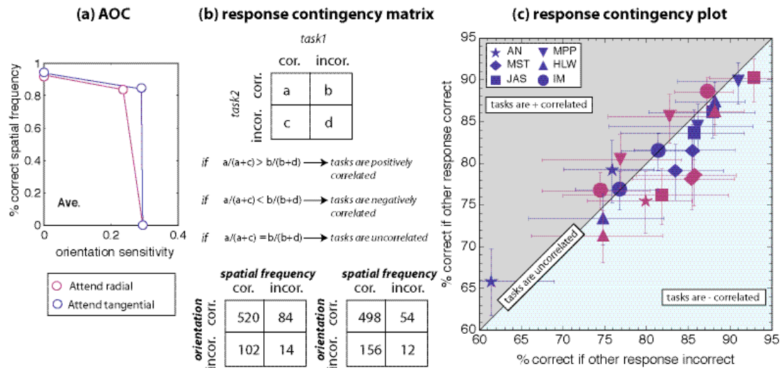
Figure 4. Average attention operating curves and error contingency analysis. (a). AOC curves. Data points on the horizontal axis illustrate single-task orientation sensitivities (1/threshold). Points on the vertical axis illustrate single-task spatial frequency discriminations. Points inside the graph illustrate dual-task performances. (b) Error contingency analysis. Inequalities derived from the four possible response categories reveal whether performance on task 1 is positively correlated, negatively correlated or uncorrelated with performance on task 2. Two separate contingency analyses were performed for each observer in each dual-task condition; once using the primary (orientation) task as “task 1,” and once using it as “task 2.” An example is given at the bottom for observer JAS in the attend-tangential condition (left) and attend-radial condition (right). Accuracy on task 1 is plotted in (c). Red symbols illustrate the attend-radial condition, blue symbols illustrate the attend-tangential condition. Symbols in the grey area indicate positively correlated performances, whereas symbols in the blue area indicate negatively correlated performances. Error bars contain 95% (binomial) confidence intervals.
