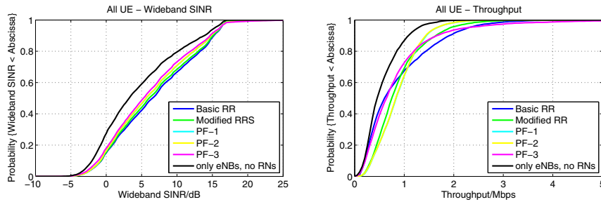
Figure 5. SLS Results for all UEs served by eNBs and RNs
