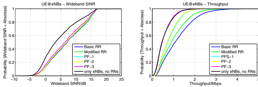
Figure 3. SLS Results for UEs served by eNBs
