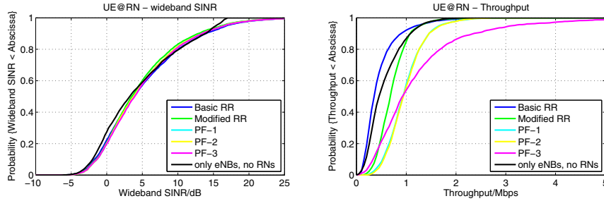
Figure 4. SLS Results for UEs served by RNs
