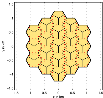
Figure 2. Network Layout, 19 eNBs, 3 Sectors/Site, 4 RNs per Sector
