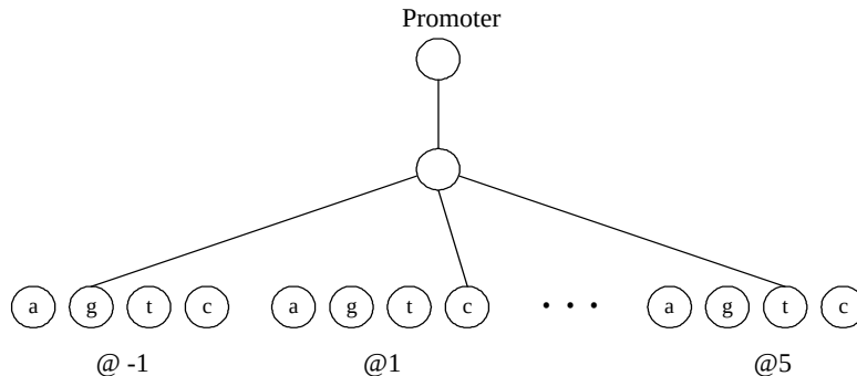
Figure 21: Part of the network for Promoter Recognition.
