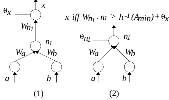
Figure 4: A single hidden neuron network (1) and its associated constraint (2) w.r.t. output x . W_a, W_b, W_{n_1} \in \mathbb{R}^+ .
