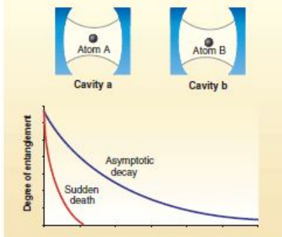
Fig. 1. Curves show ESD as one of two routes for relaxation of the entanglement, via concurrence C(\rho) , of qubits A and B that are located in separate overlapped cavities.
