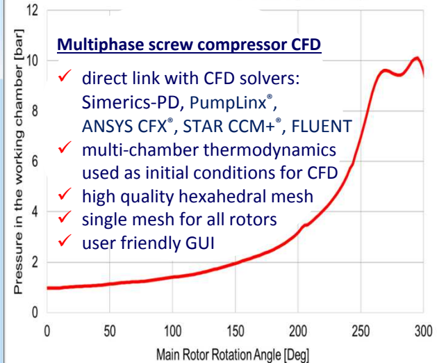
CFD - oil injected air screw compressor 6000 rpm; 1b & 20°C suction; 8b discharge
